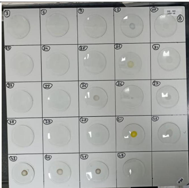
Test set up for Chemical Spot Test(Method B)
